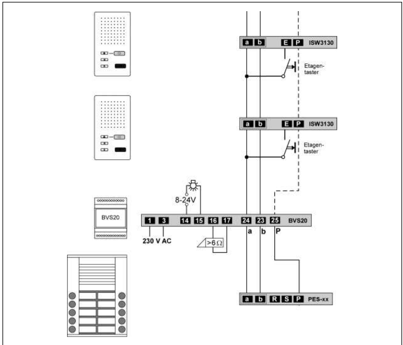
Connection diagram 2-wire technique
